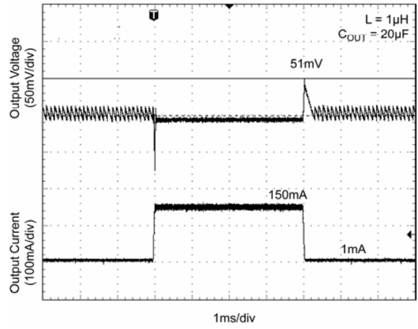
Transient Response
